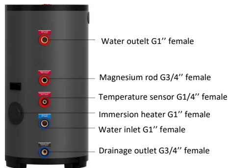
Left View
